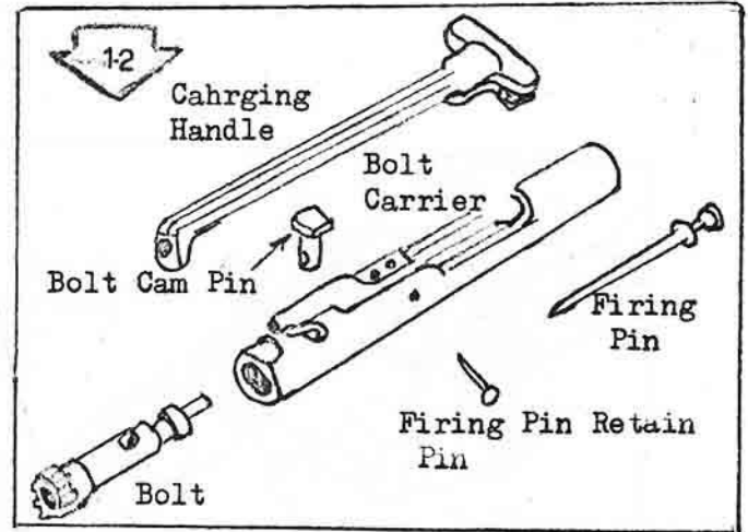
BOLT CARRIER GROUP PARTS
